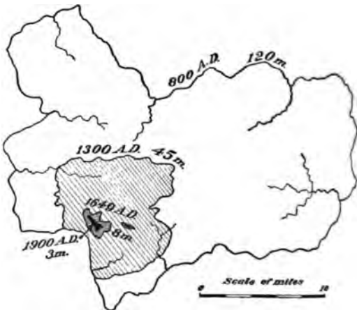
FIG. 256.—Map showing the outlines of the Island of Heligoland at different stages in its recent history. The peripheries given are in miles.
